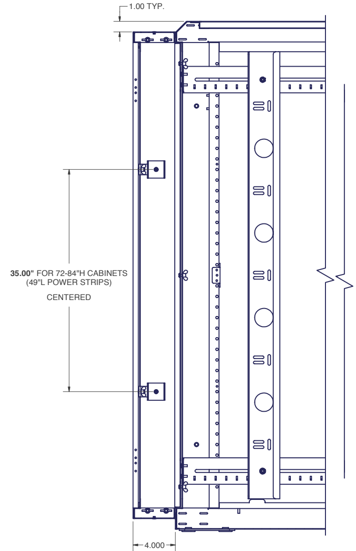
SECTION B-B
