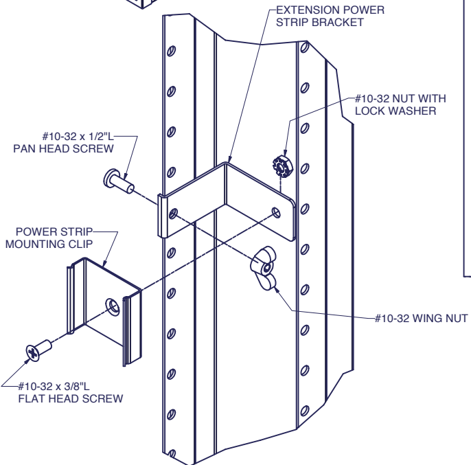
DETAIL C TYP. 2 PER EXTENSION SIDE
