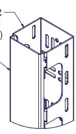
DETAIL C
