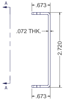
VIEW A-A (ENLARGED)
