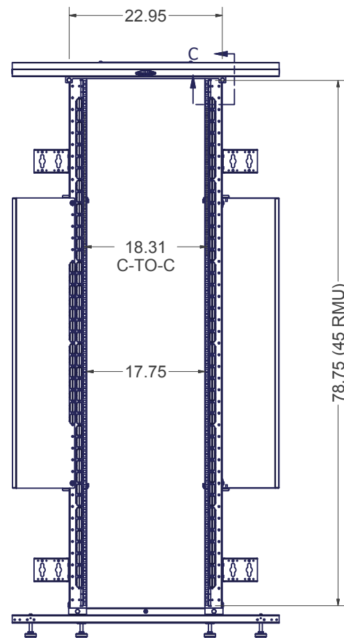
FRONT VIEW DOORS AND SIDES REMOVED
