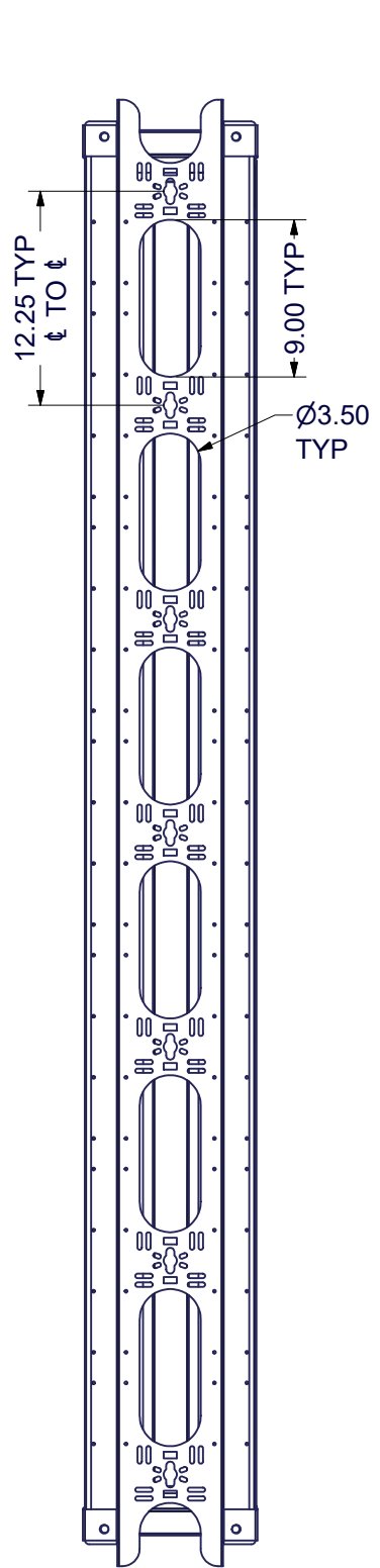
REAR VIEW
