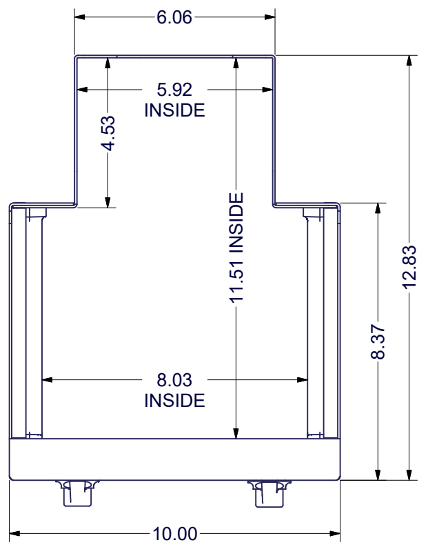
VIEW A-A TOP VIEW
