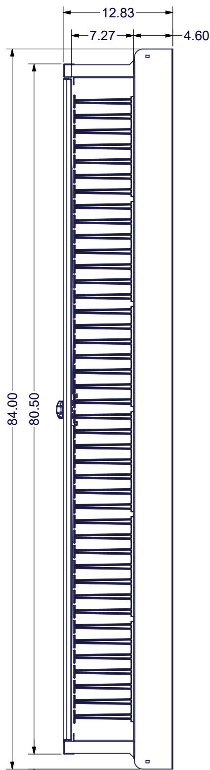
SIDE VIEW 1.75 FLOATING OFF THE FLOOR
