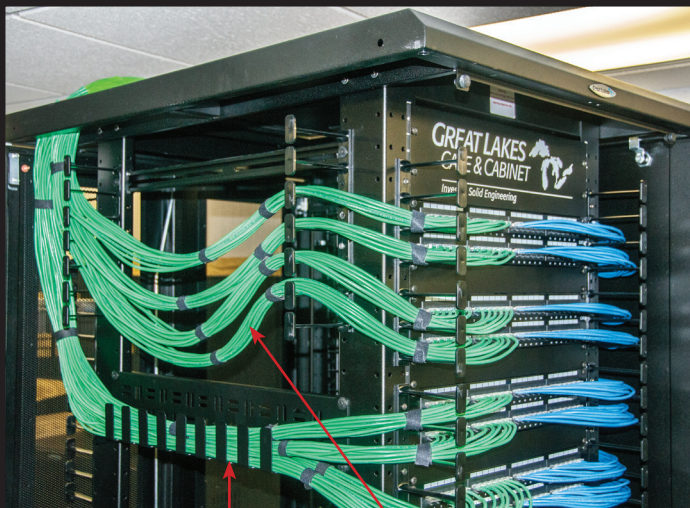
Use of the Horizontal Cable Manager
