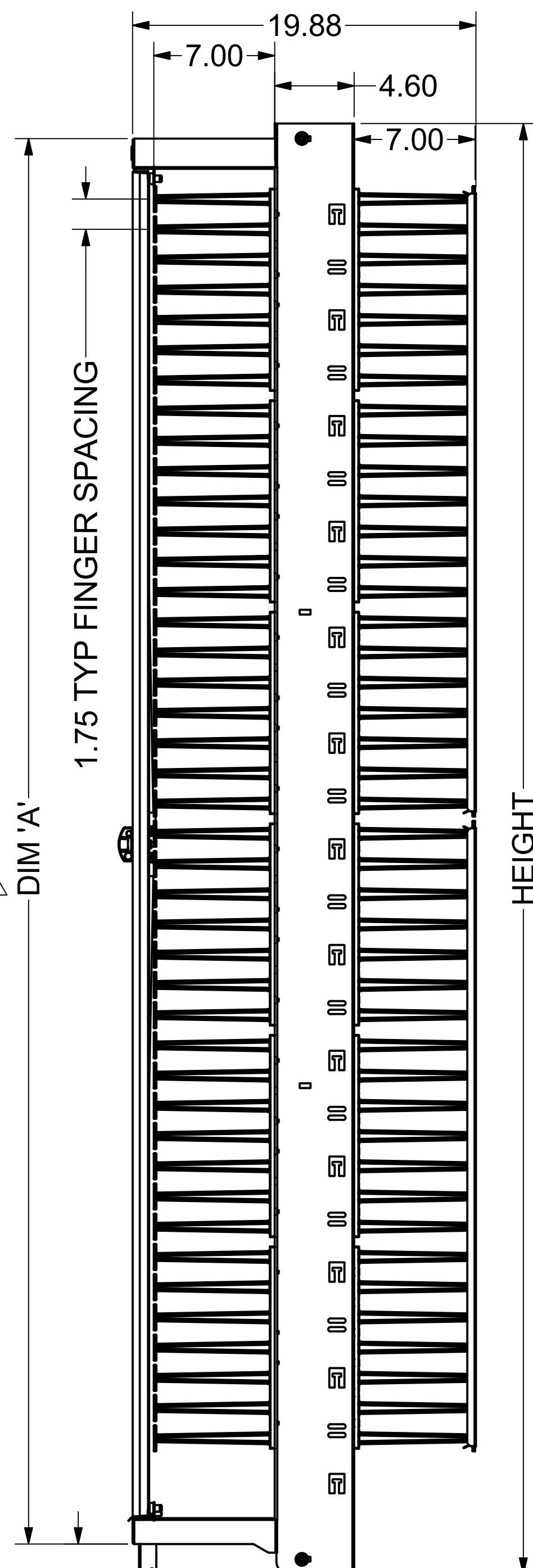
SIDE VIEW
