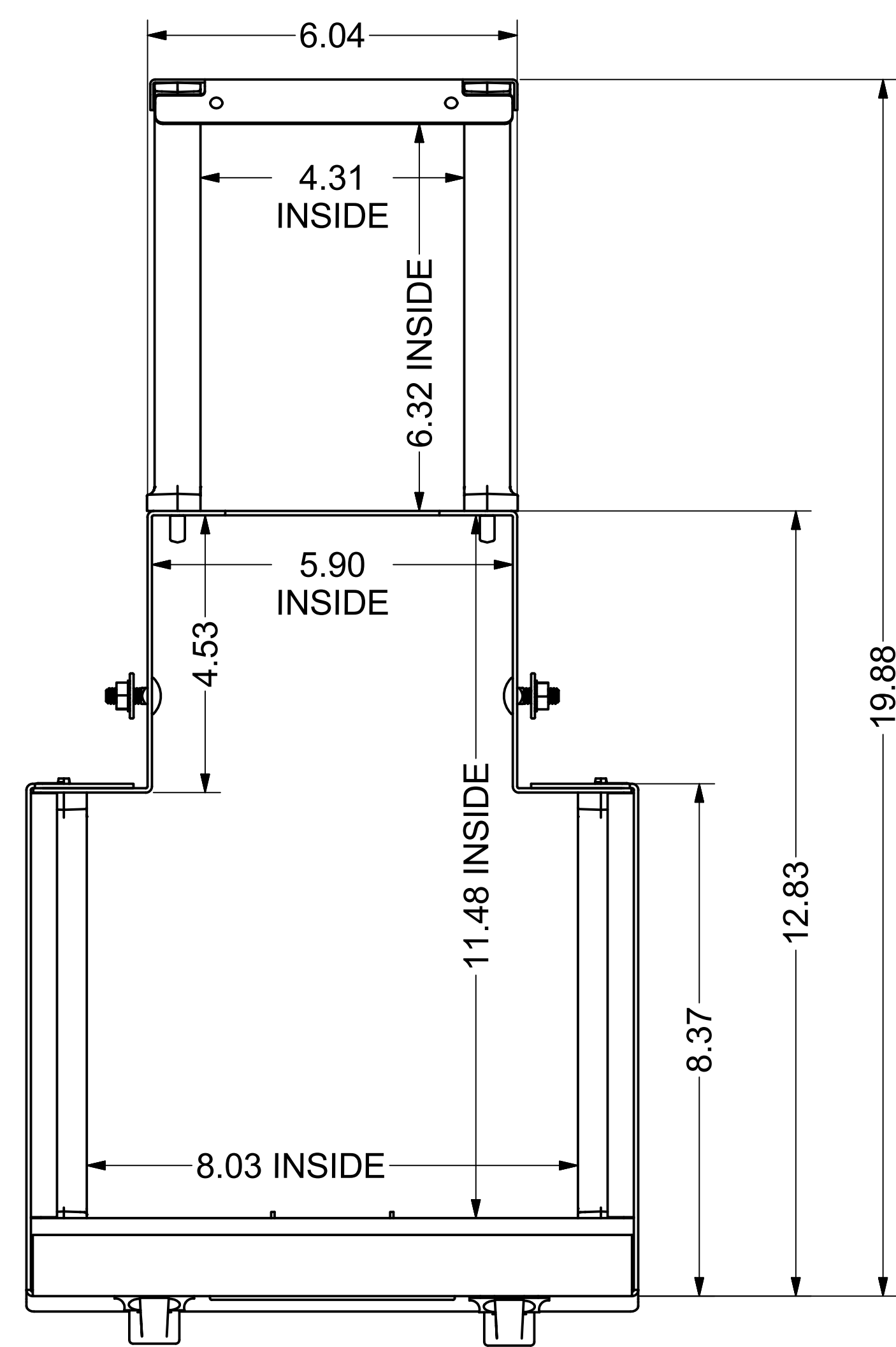
VIEW A-A TOP VIEW
